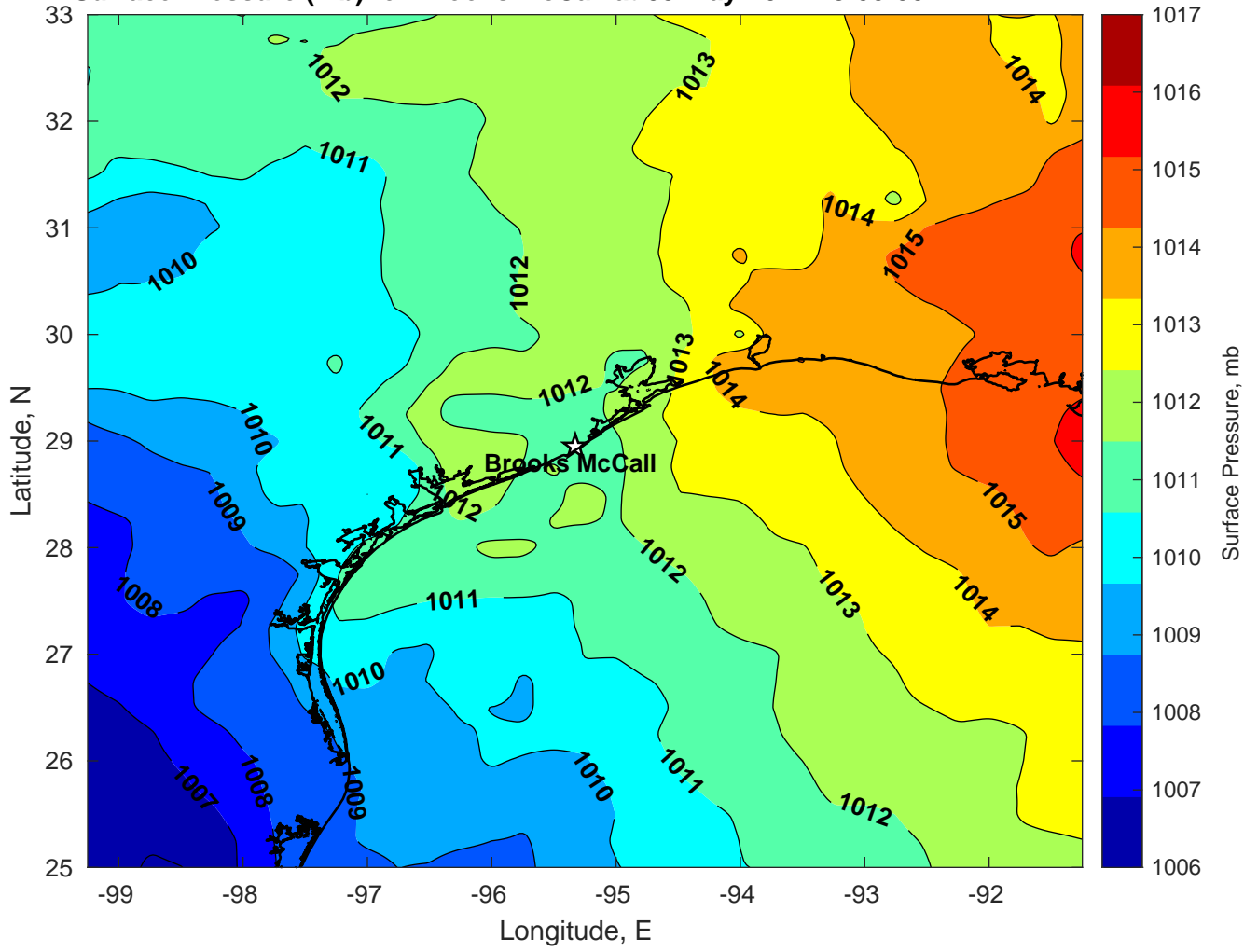
Surface Pressure (mb) for Brooks McCall at 05-May-2024 18:00:00
